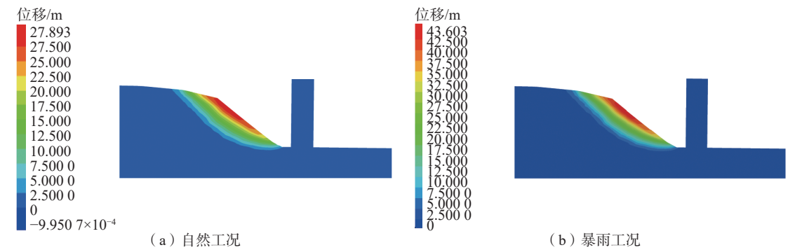
图 15 不同工况下斜坡水平位移云图 Fig. 15 Horizontal displacement contour map of slopes under different working conditions
