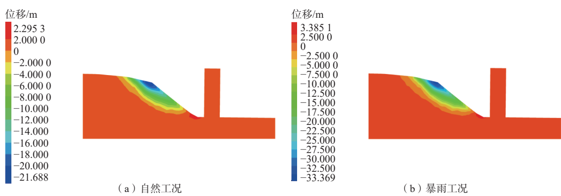
图 16 不同工况下斜坡垂直位移云图 Fig. 16 Vertical displacement contour maps of slopes under different operating conditions
