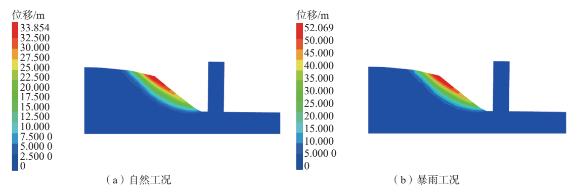
图 17 不同工况下斜坡总位移云图 Fig. 17 Total displacement contour map of slopes under different operating conditions
