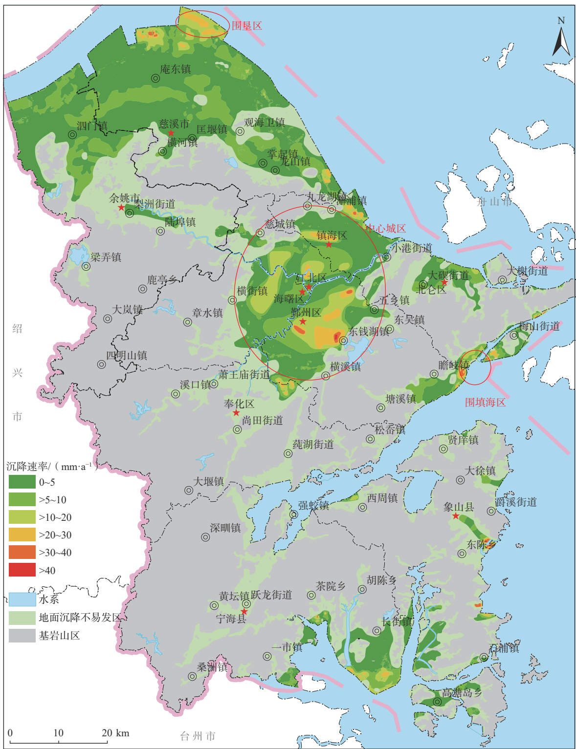
图 1 宁波市地面沉降速率概况 Fig. 1 Overview of land subsidence rates in Ningbo City
