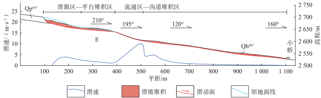
图 10 永光 1#滑坡滑速分析图 Fig. 10 Analysis of the sliding speed of the Yongguang 1# landslide
