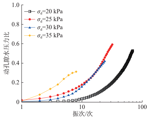
图 12 滑体土动三轴试验曲线图 Fig. 12 Dynamic triaxial test curve of the sliding soil
