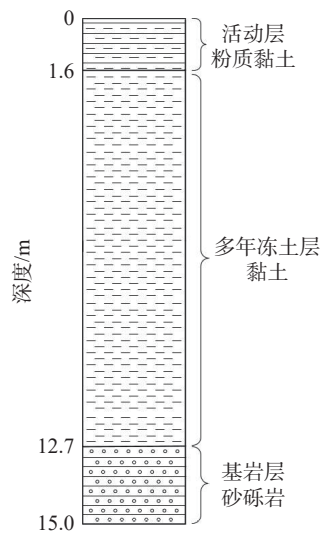
图 3 钻孔地层信息(水) Fig. 3 Stratum information based on borehole
