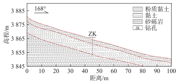
图 4 典型斜坡地质剖面 Fig. 4 Typical geological section of the slope
