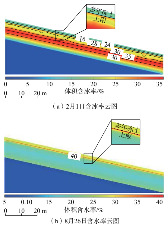
图 8 斜坡含水率和含冰率分布规律 Fig. 8 Water content and ice content distribution law of slope
