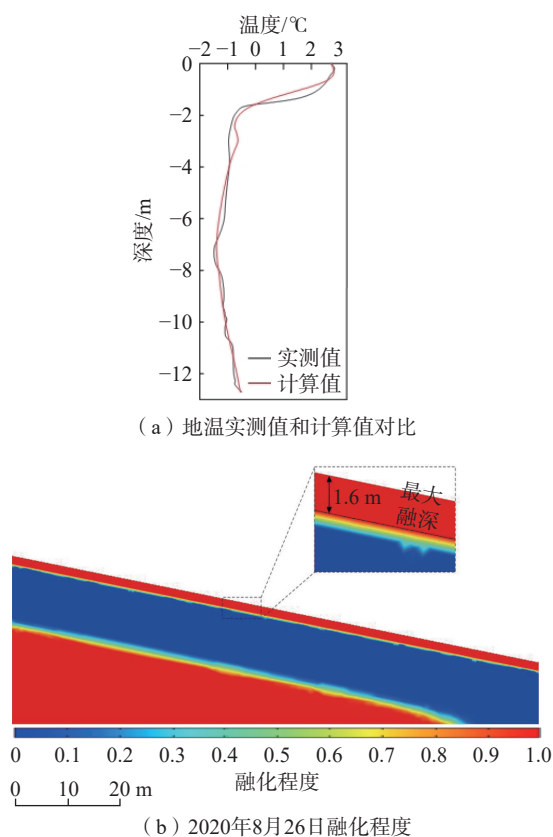
图 6 模型有效性验证 Fig. 6 Effectiveness verification of model
